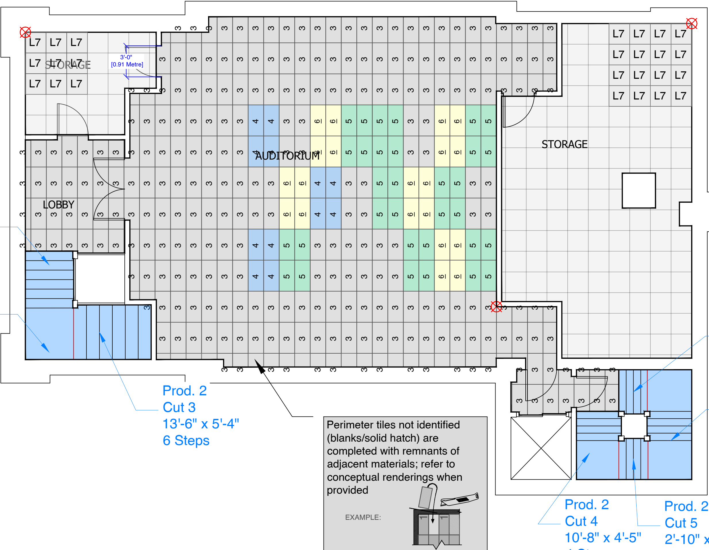
3 SECOND FLOOR PLAN 3/16" = 1'-0"
