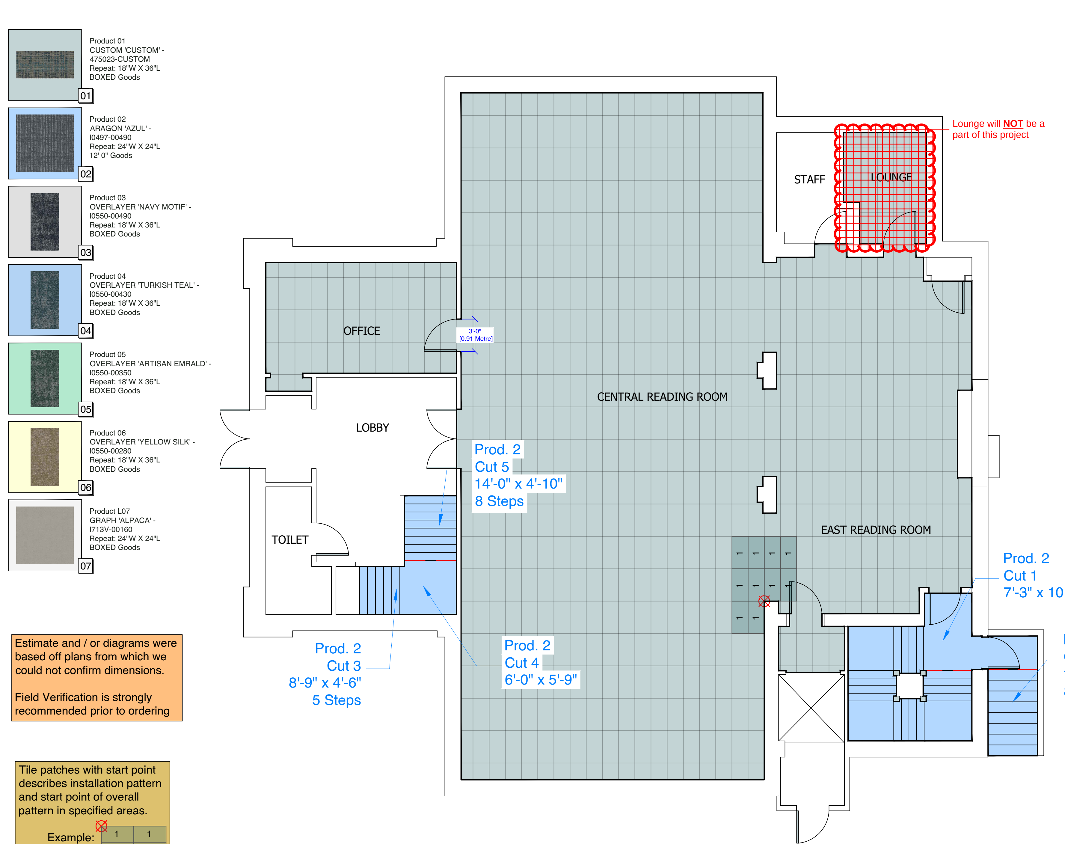
1 FIRST FLOOR PLAN 3/16" = 1'-0"
